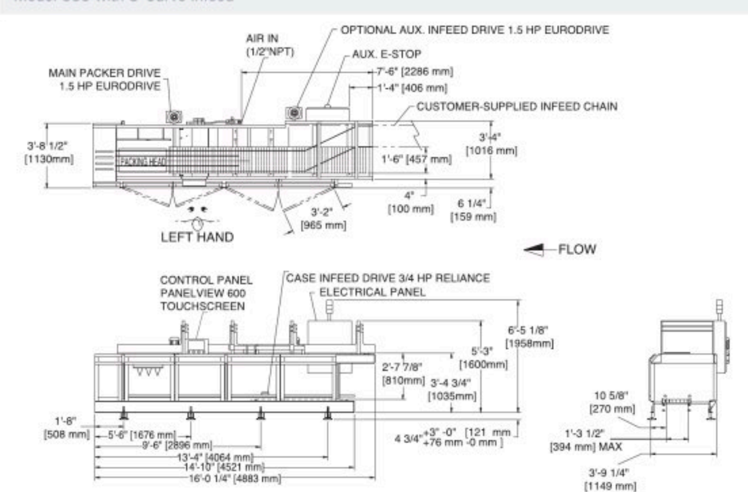
Model 835 with S-Curve Infeed
